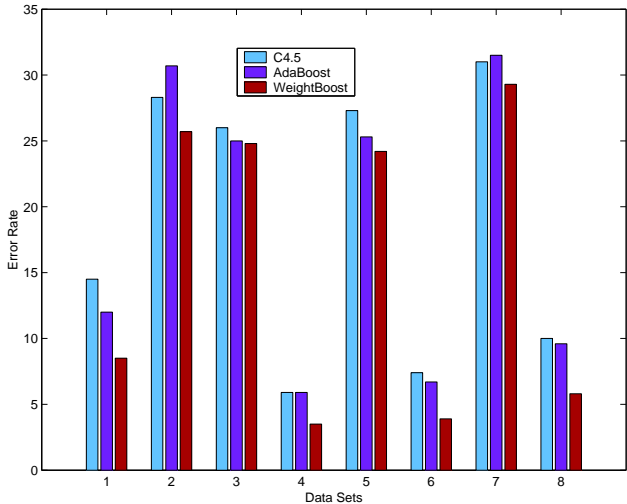
Figure 1. Classification Errors with 10% Noise
