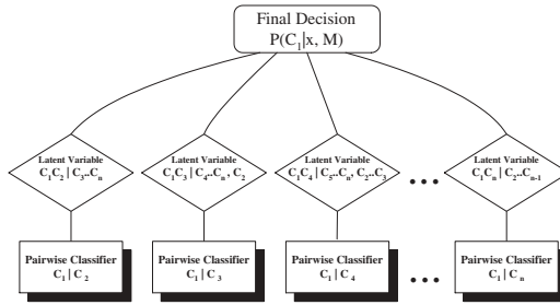
Fig. 2. The Structure of the Pairwise Ensemble Approach for Class C_1 .
